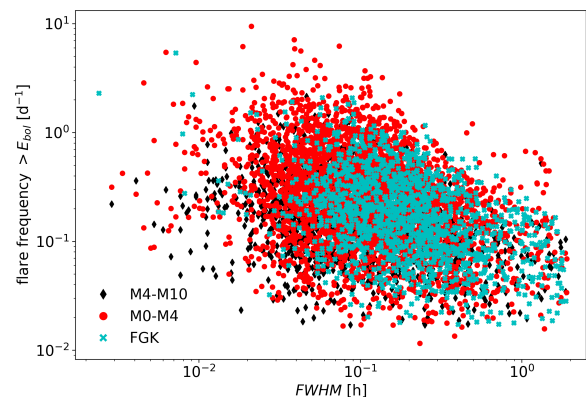
FIGURE 2 Flare frequency above bolometric flare energy E_{bol} in flare stars with flares with measured FWHM . Note that the frequencies are for individual stars that were caught flaring within the first two Sectors of TESS Cycle 1 by Günther et al. (2020). Stars that flare but did not show any flares within the two first Sectors are not included.
